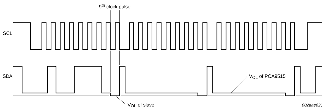
Fig 6. Bus 1 waveform
